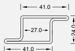
Z - SECTION - 41 x 24 mm
