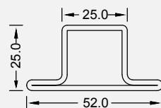
T - SECTION - 52 x 25 mm
